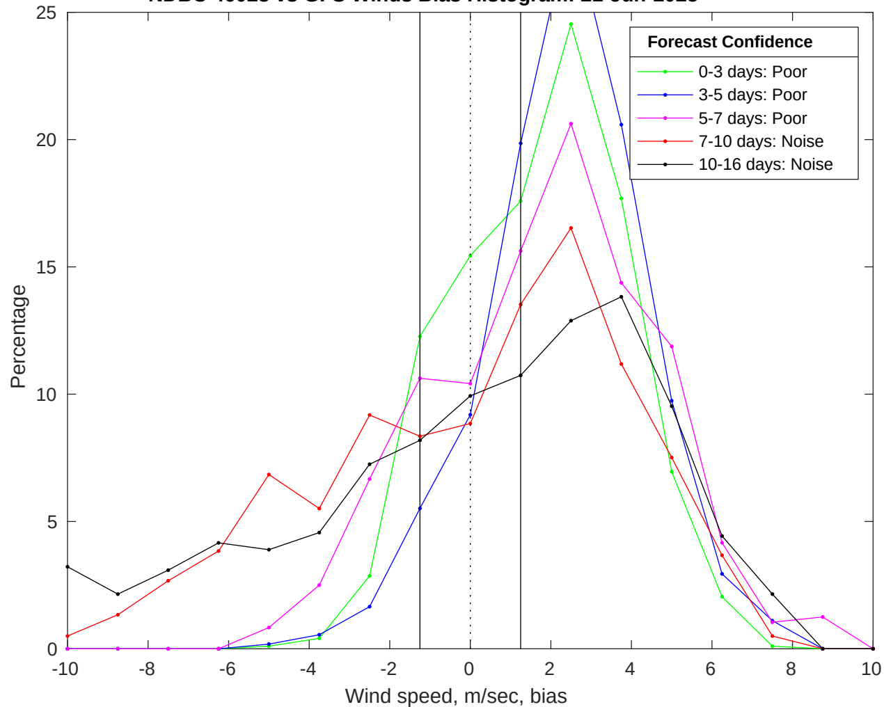
NDBC 46028 vs GFS Winds Bias Histogram: 21-Jun-2025
