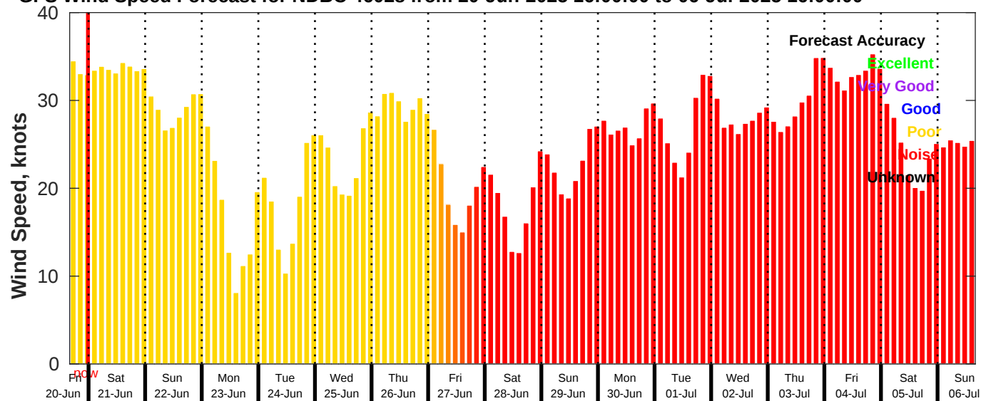
GFS Wind Speed Forecast for NDBC 46028 from 20-Jun-2025 16:00:00 to 06-Jul-2025 16:00:00
