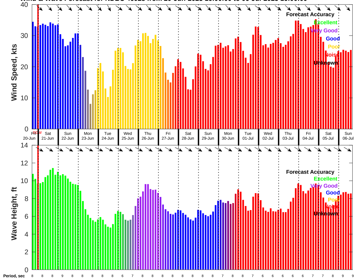
Wind & Wave Forecast for NDBC 46028 from 20-Jun-2025 16:00:00 to 06-Jul-2025 16:00:00
