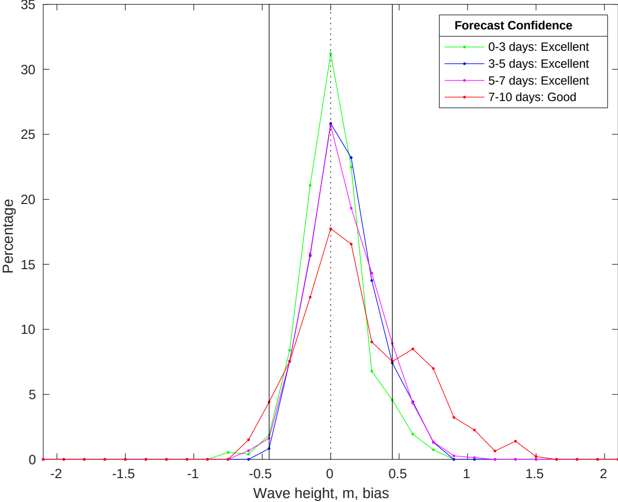
NDBC 46054 vs CMEMS Waves Bias Histogram: 21-Jun-2025
