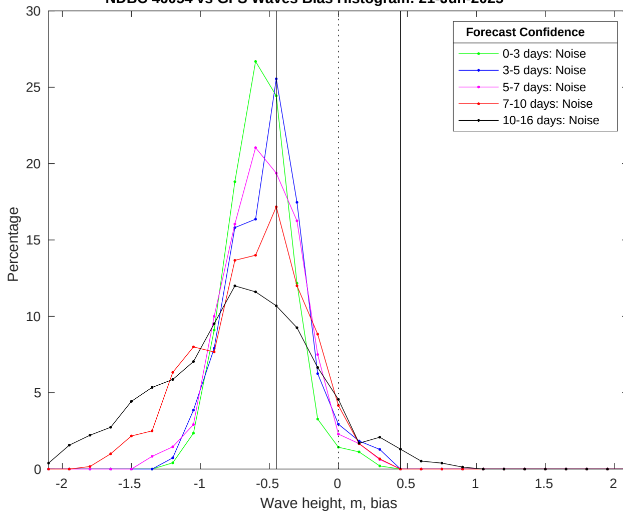
NDBC 46054 vs GFS Waves Bias Histogram: 21-Jun-2025
