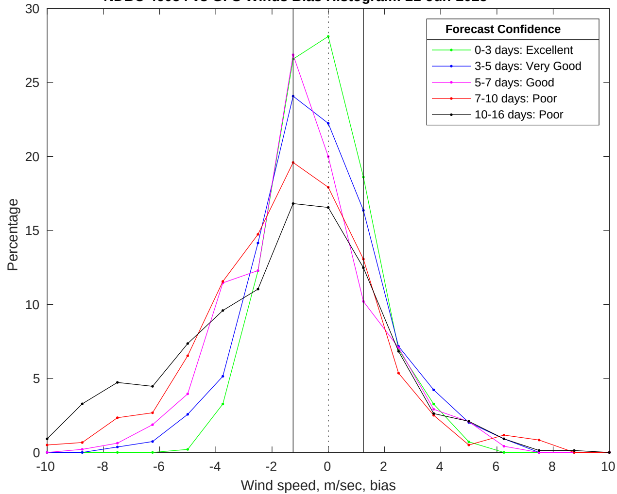
NDBC 46054 vs GFS Winds Bias Histogram: 21-Jun-2025
