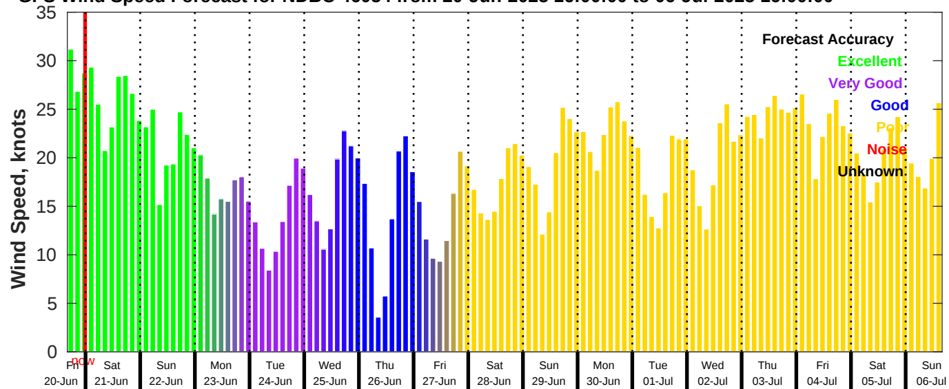
GFS Wind Speed Forecast for NDBC 46054 from 20-Jun-2025 16:00:00 to 06-Jul-2025 16:00:00
