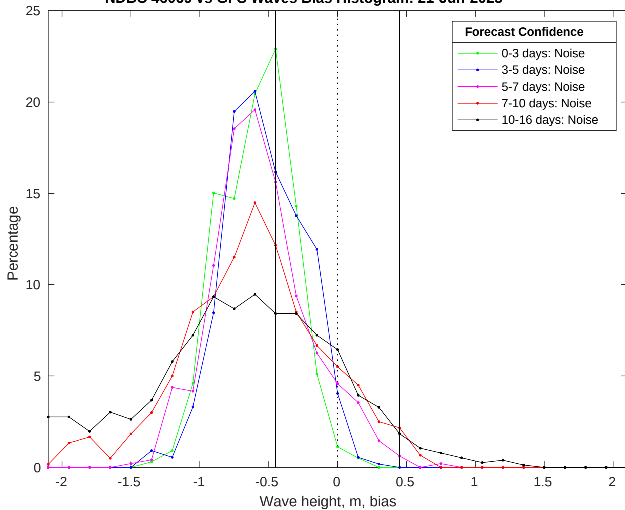
NDBC 46069 vs GFS Waves Bias Histogram: 21-Jun-2025
