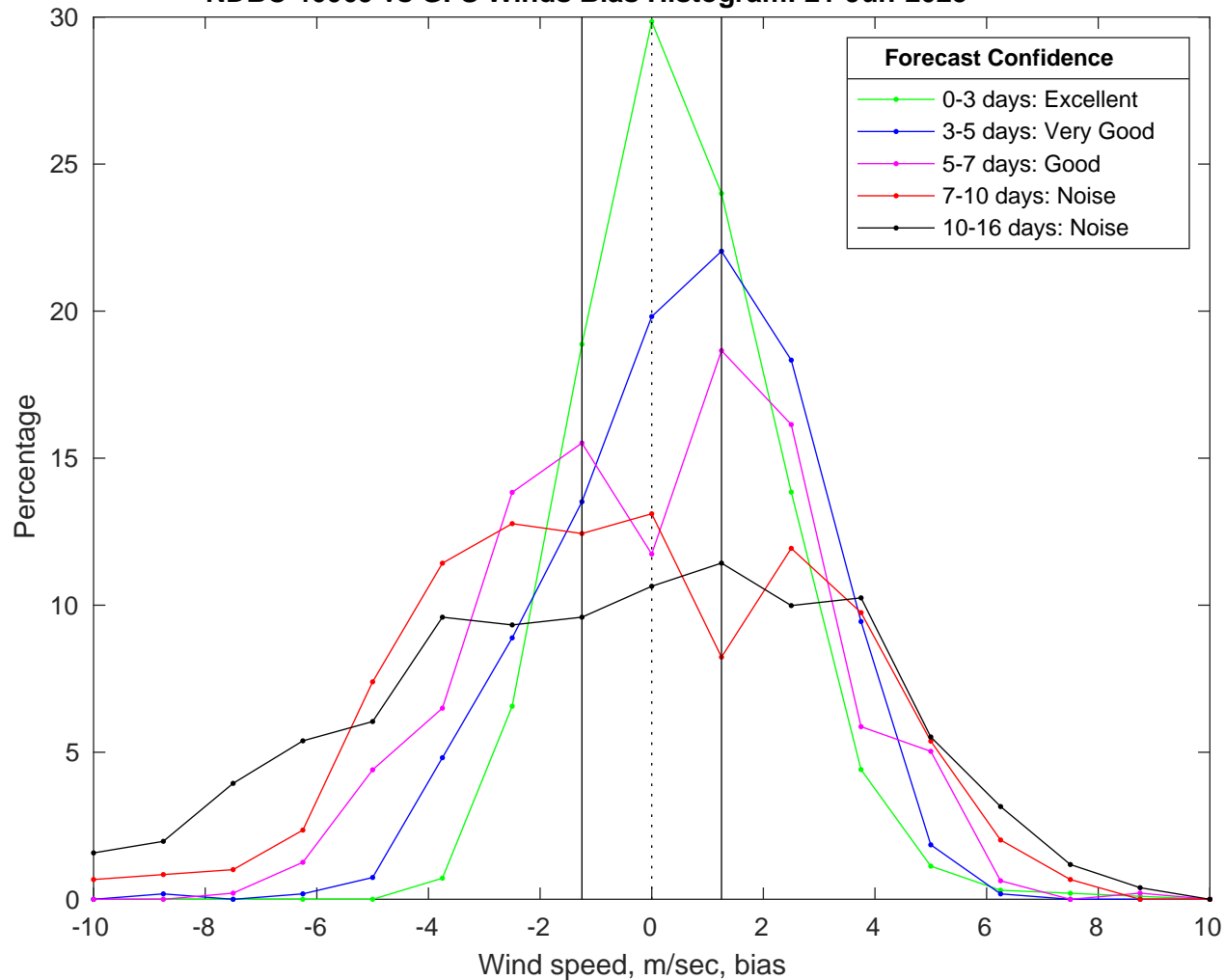
NDBC 46069 vs GFS Winds Bias Histogram: 21-Jun-2025
