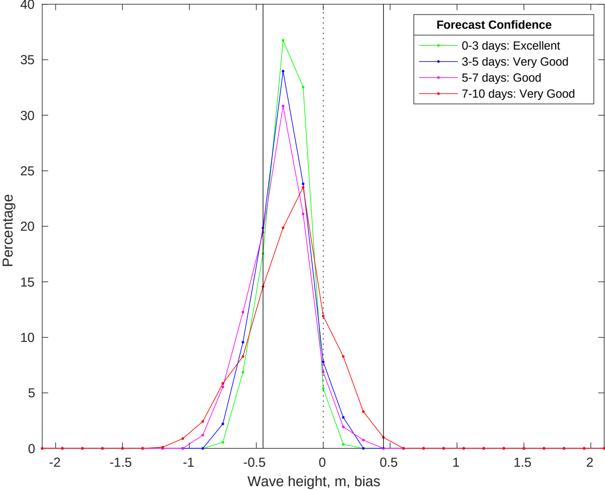
NDBC 51209 vs CMEMS Waves Bias Histogram: 21-Jun-2025
