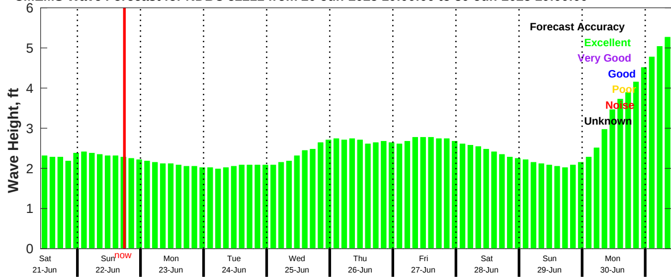
CMEMS Wave Forecast for NDBC 52211 from 20-Jun-2025 10:00:00 to 30-Jun-2025 10:00:00
