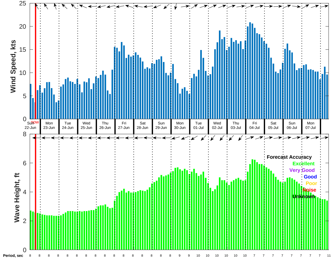
Wind & Wave Forecast for NDBC 52211 from 21-Jun-2025 10:00:00 to 07-Jul-2025 10:00:00
