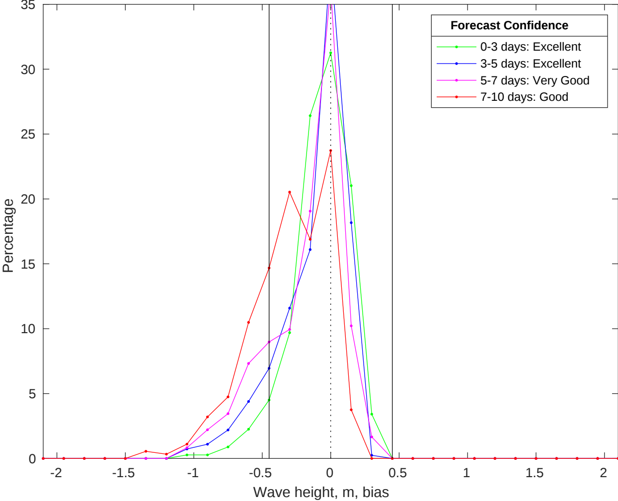
NDBC 52212 vs CMEMS Waves Bias Histogram: 21-Jun-2025
