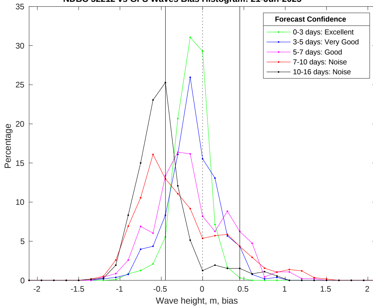
NDBC 52212 vs GFS Waves Bias Histogram: 21-Jun-2025
