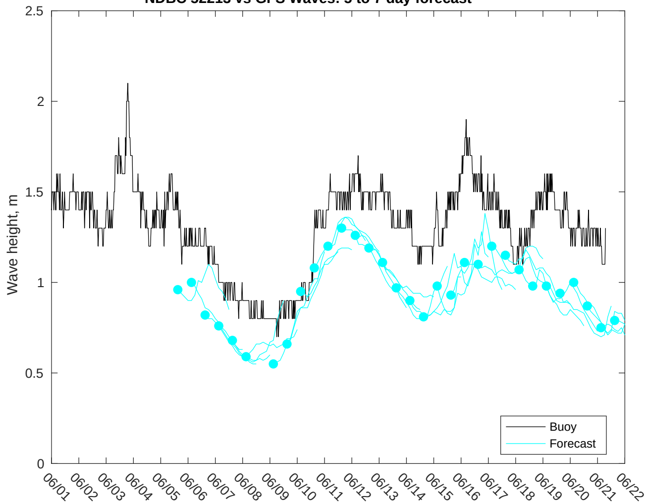
NDBC 52213 vs GFS Waves: 5 to 7 day forecast
