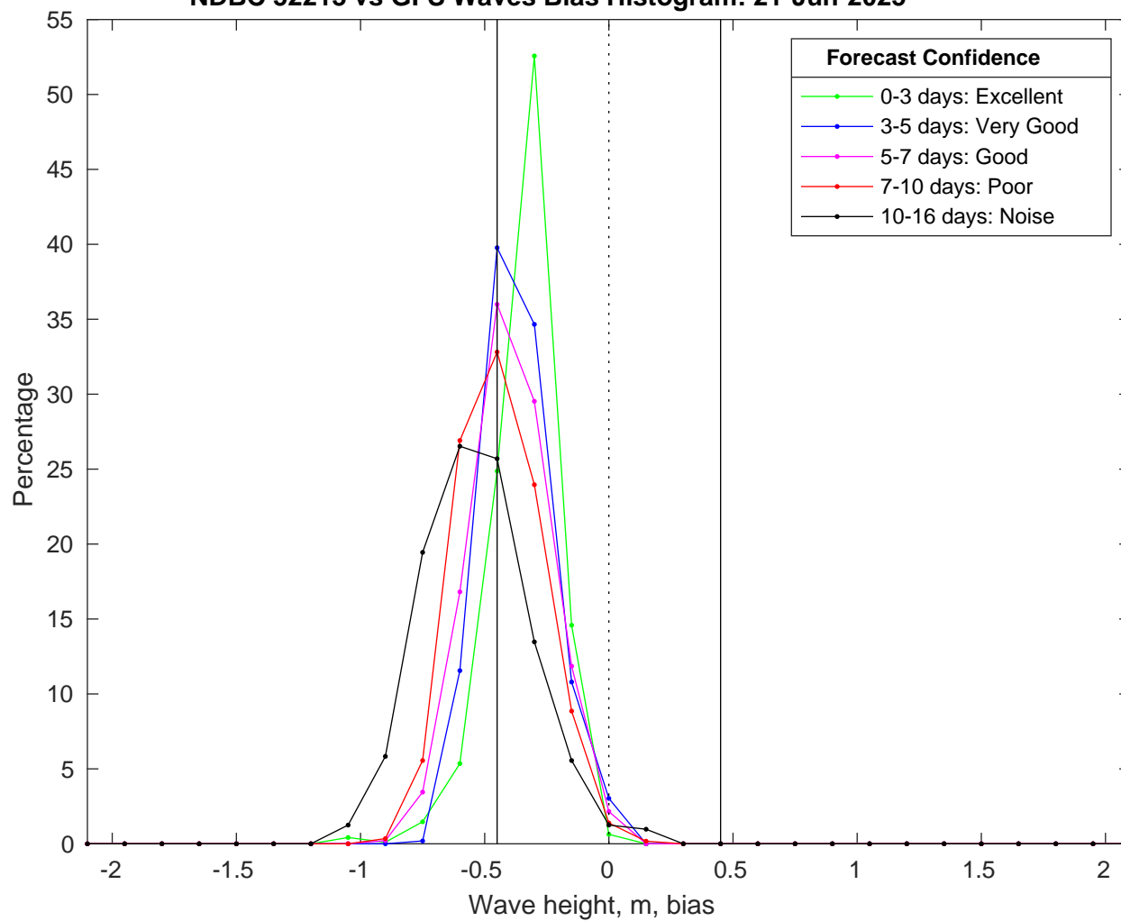
NDBC 52213 vs GFS Waves Bias Histogram: 21-Jun-2025
