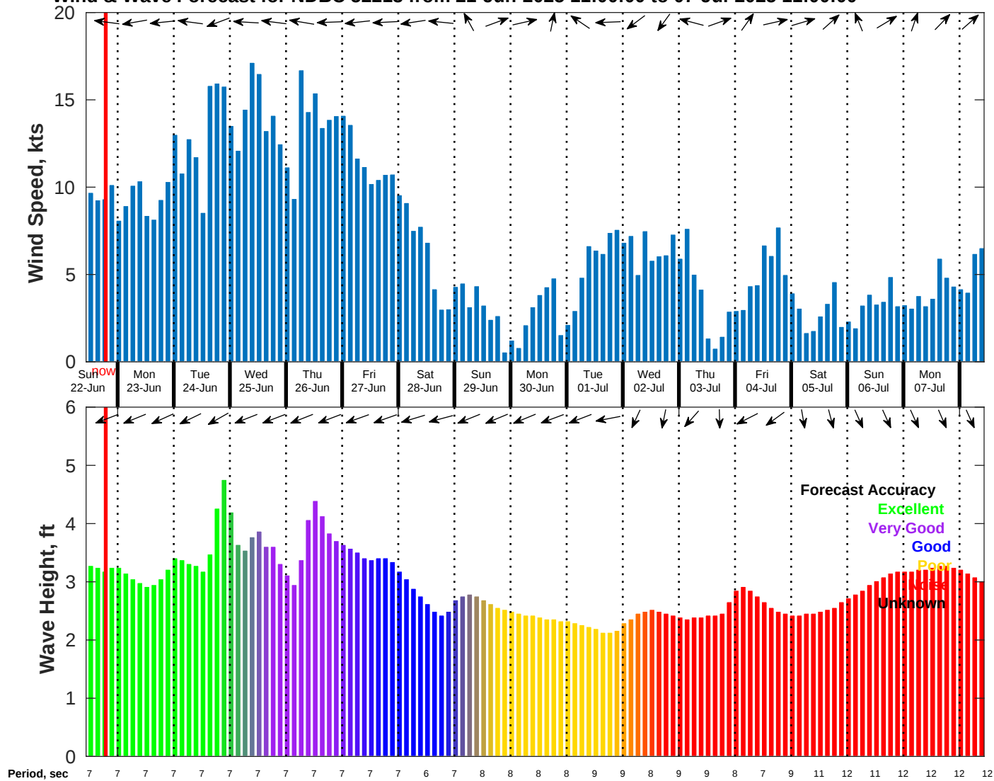
Wind & Wave Forecast for NDBC 52213 from 21-Jun-2025 11:00:00 to 07-Jul-2025 11:00:00
