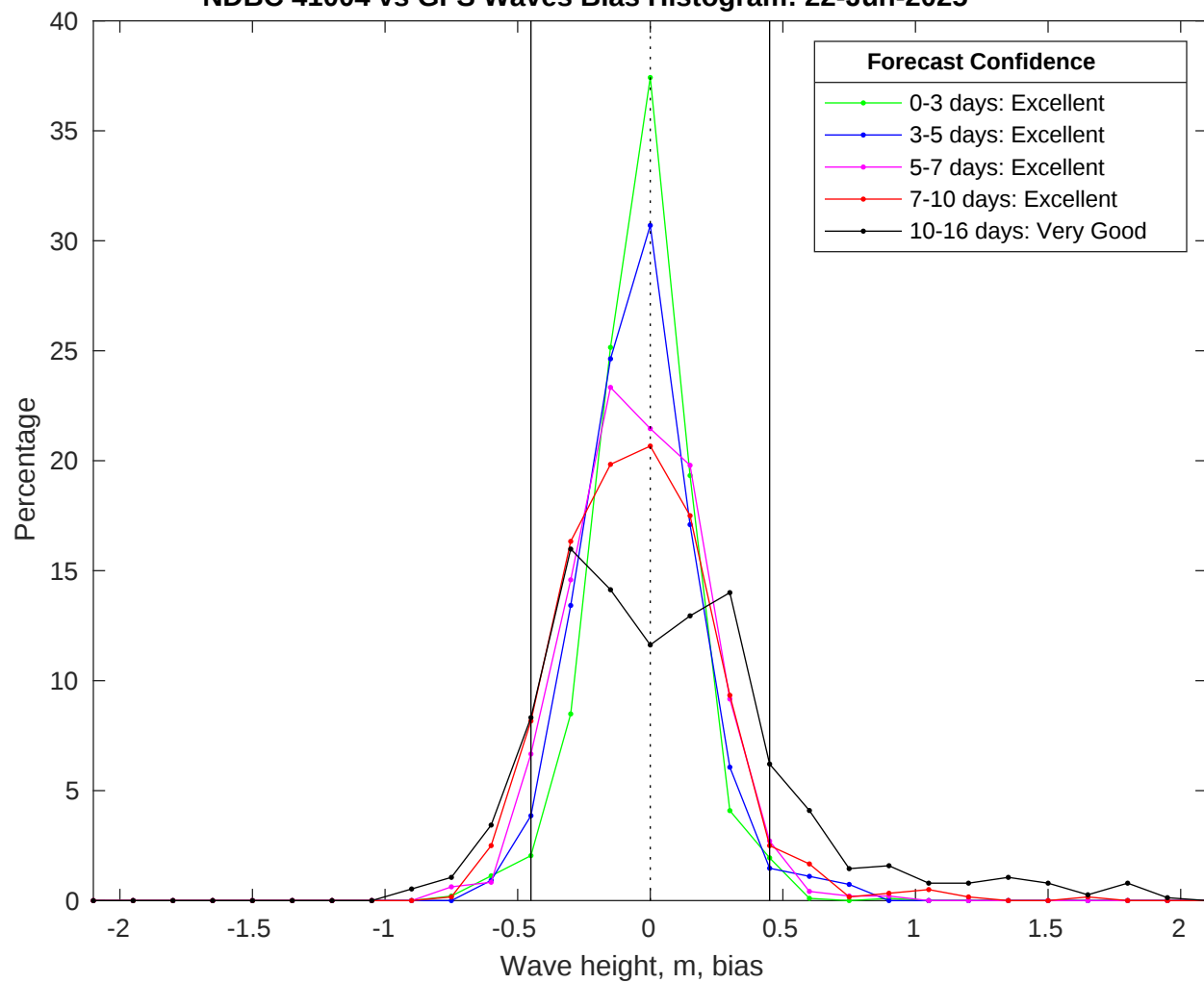
NDBC 41004 vs GFS Waves Bias Histogram: 22-Jun-2025
