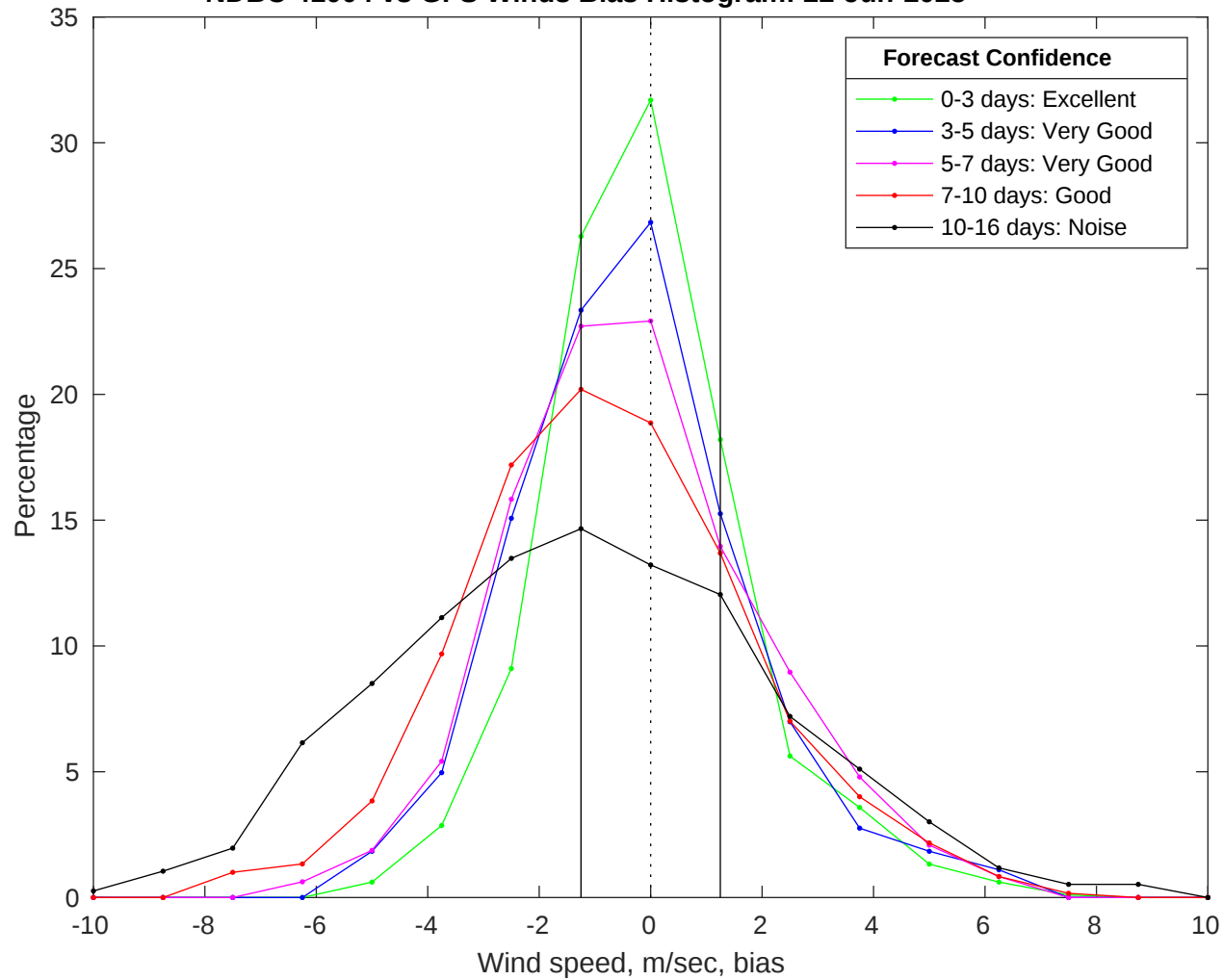
NDBC 41004 vs GFS Winds Bias Histogram: 22-Jun-2025
