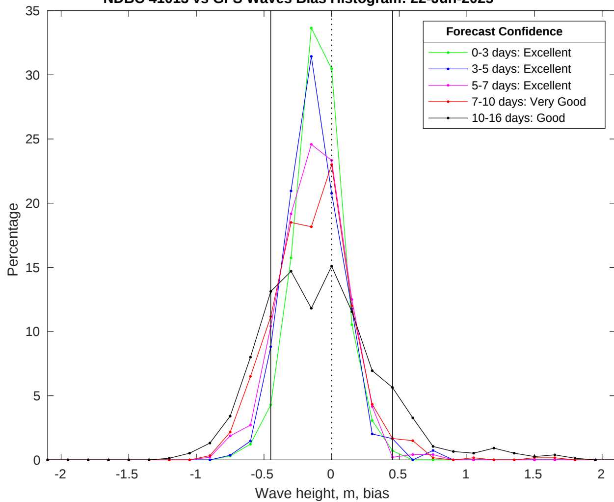
NDBC 41013 vs GFS Waves Bias Histogram: 22-Jun-2025
