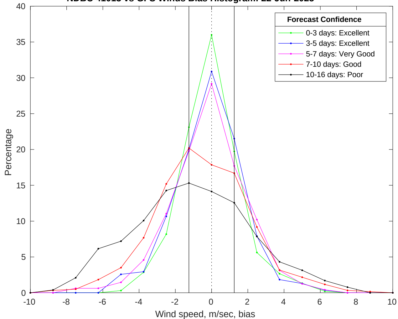
NDBC 41013 vs GFS Winds Bias Histogram: 22-Jun-2025
