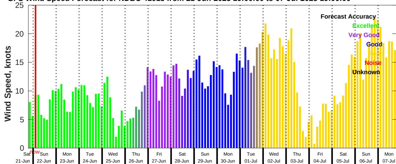
GFS Wind Speed Forecast for NDBC 41013 from 21-Jun-2025 19:00:00 to 07-Jul-2025 19:00:00
