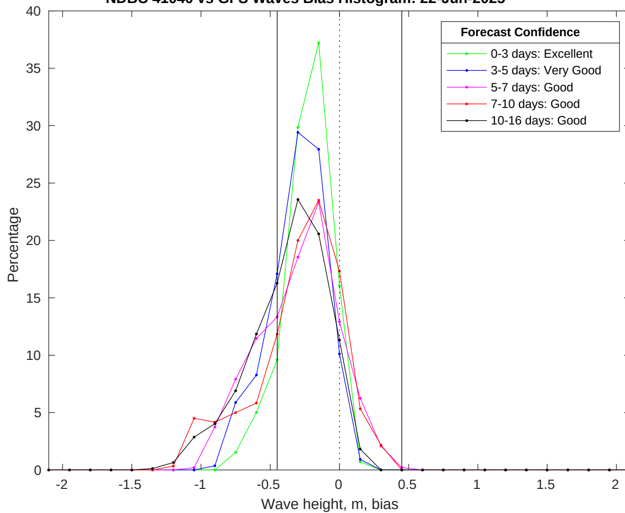
NDBC 41040 vs GFS Waves Bias Histogram: 22-Jun-2025
