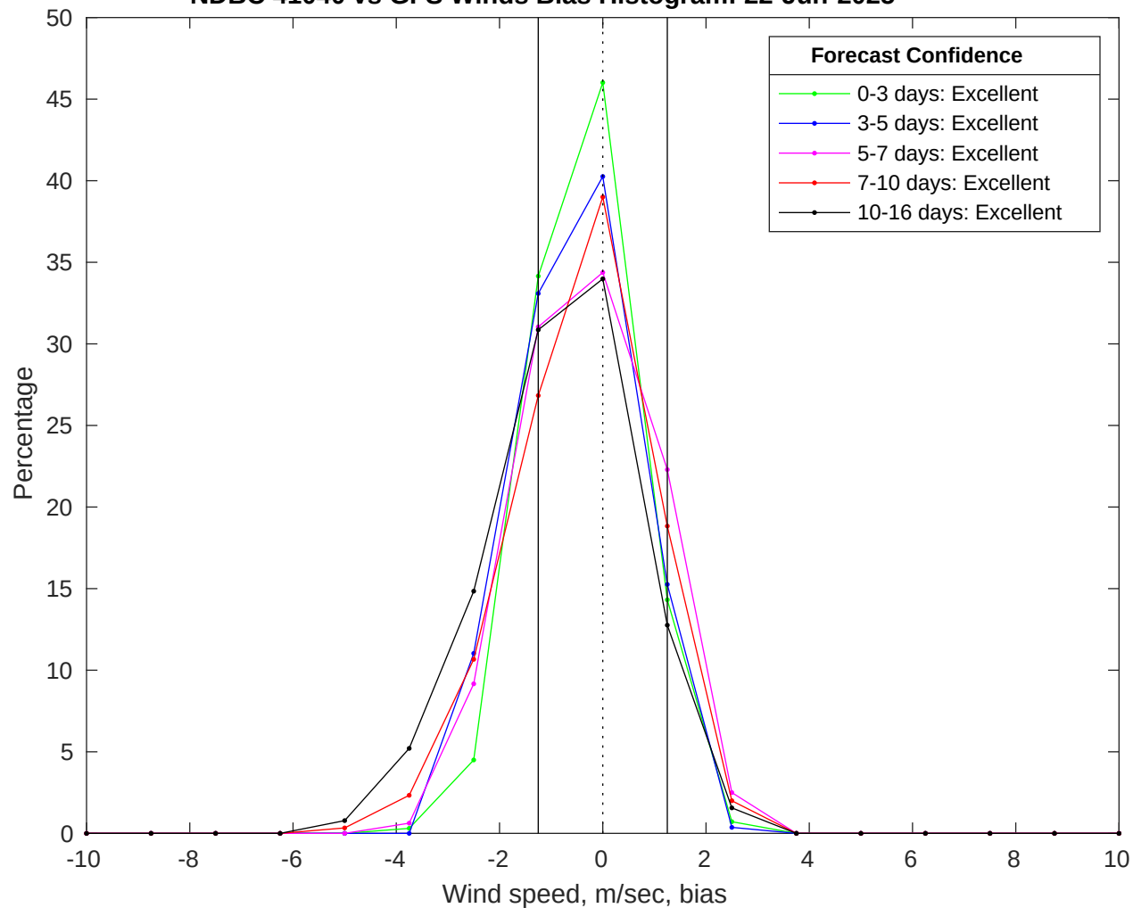
NDBC 41040 vs GFS Winds Bias Histogram: 22-Jun-2025
