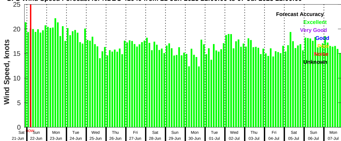
GFS Wind Speed Forecast for NDBC 41040 from 21-Jun-2025 21:00:00 to 07-Jul-2025 21:00:00
