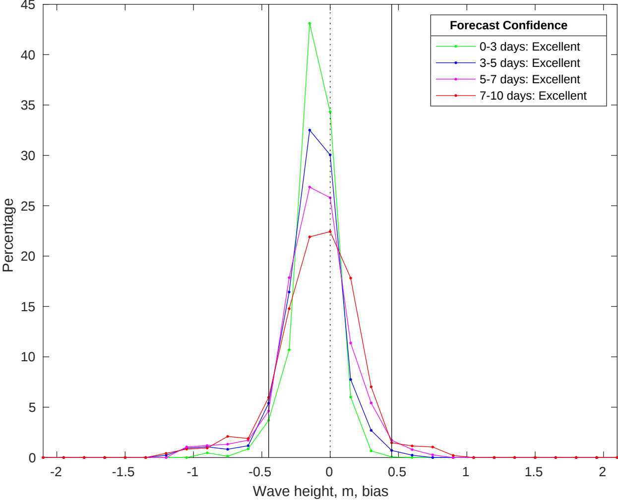
NDBC 42019 vs CMEMS Waves Bias Histogram: 22-Jun-2025
