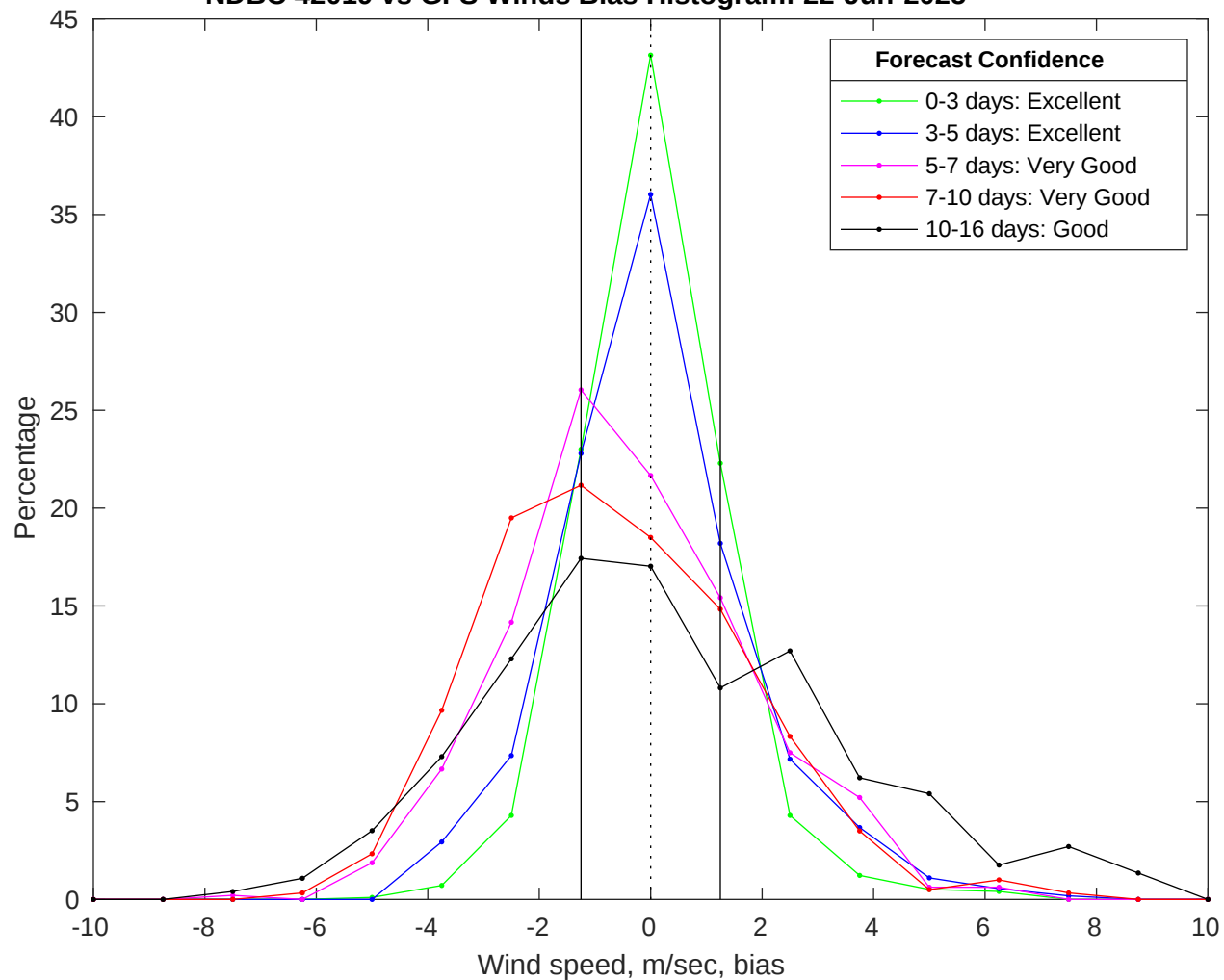
NDBC 42019 vs GFS Winds Bias Histogram: 22-Jun-2025
