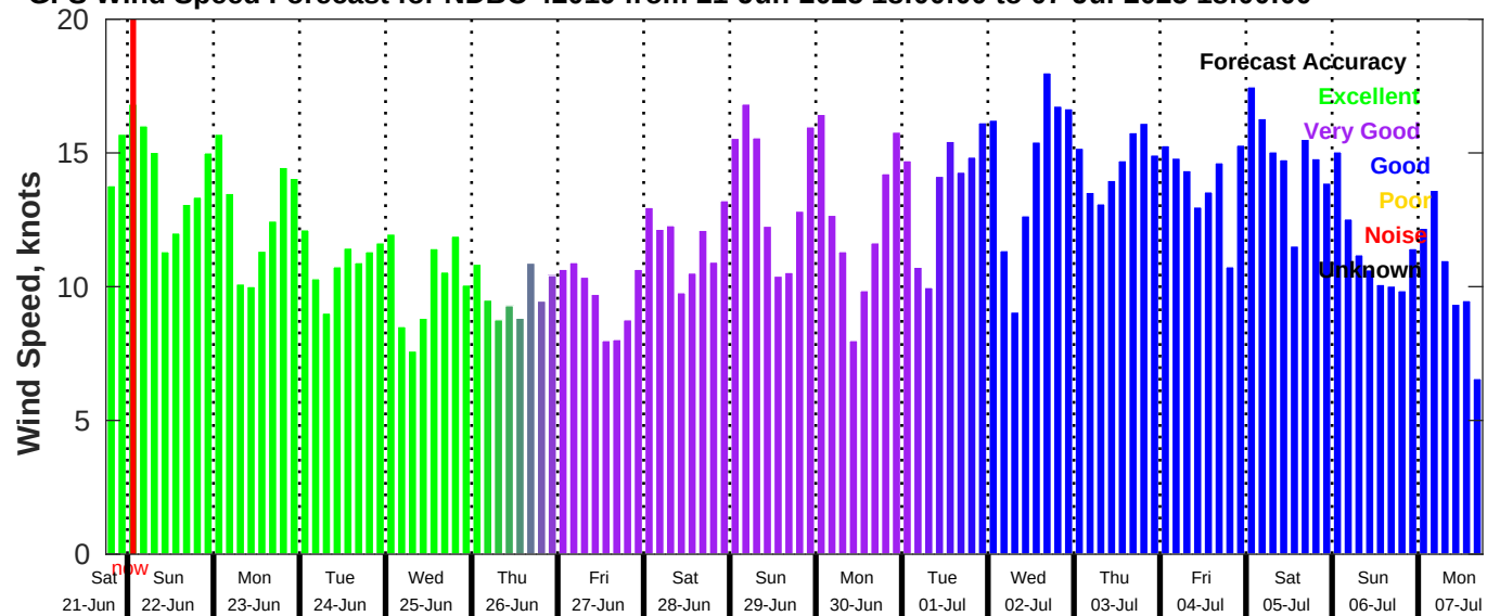
GFS Wind Speed Forecast for NDBC 42019 from 21-Jun-2025 18:00:00 to 07-Jul-2025 18:00:00
