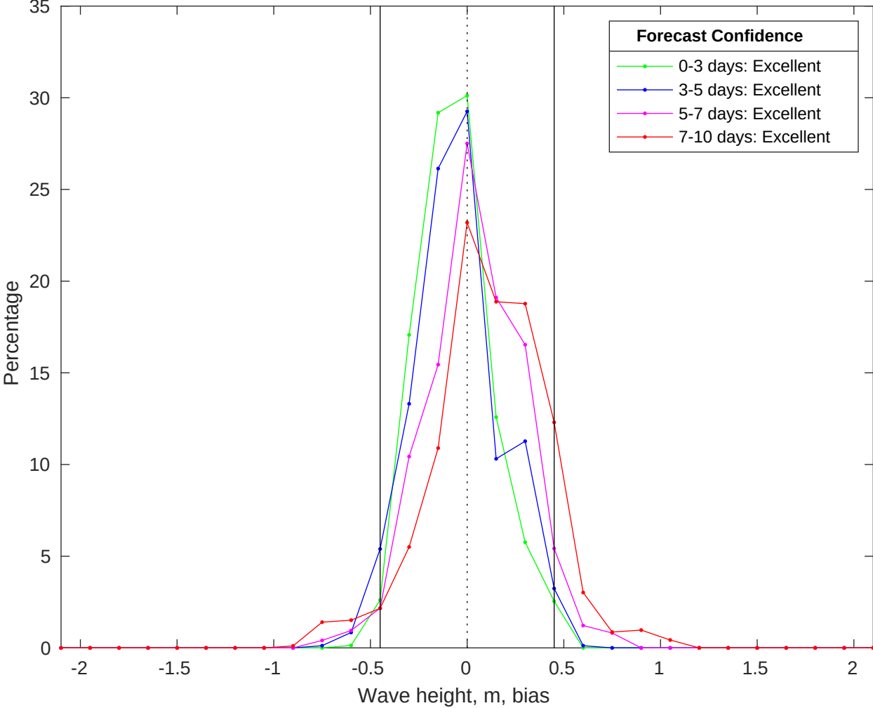
NDBC 42020 vs CMEMS Waves Bias Histogram: 21-Jun-2025
