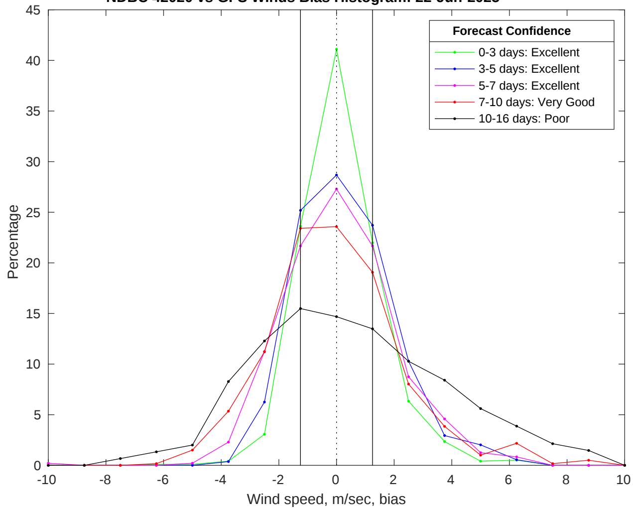
NDBC 42020 vs GFS Winds Bias Histogram: 22-Jun-2025
