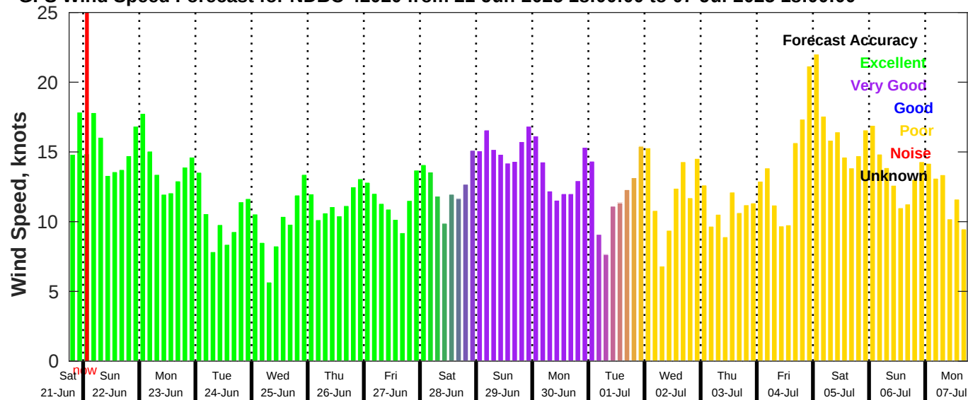
GFS Wind Speed Forecast for NDBC 42020 from 21-Jun-2025 18:00:00 to 07-Jul-2025 18:00:00
