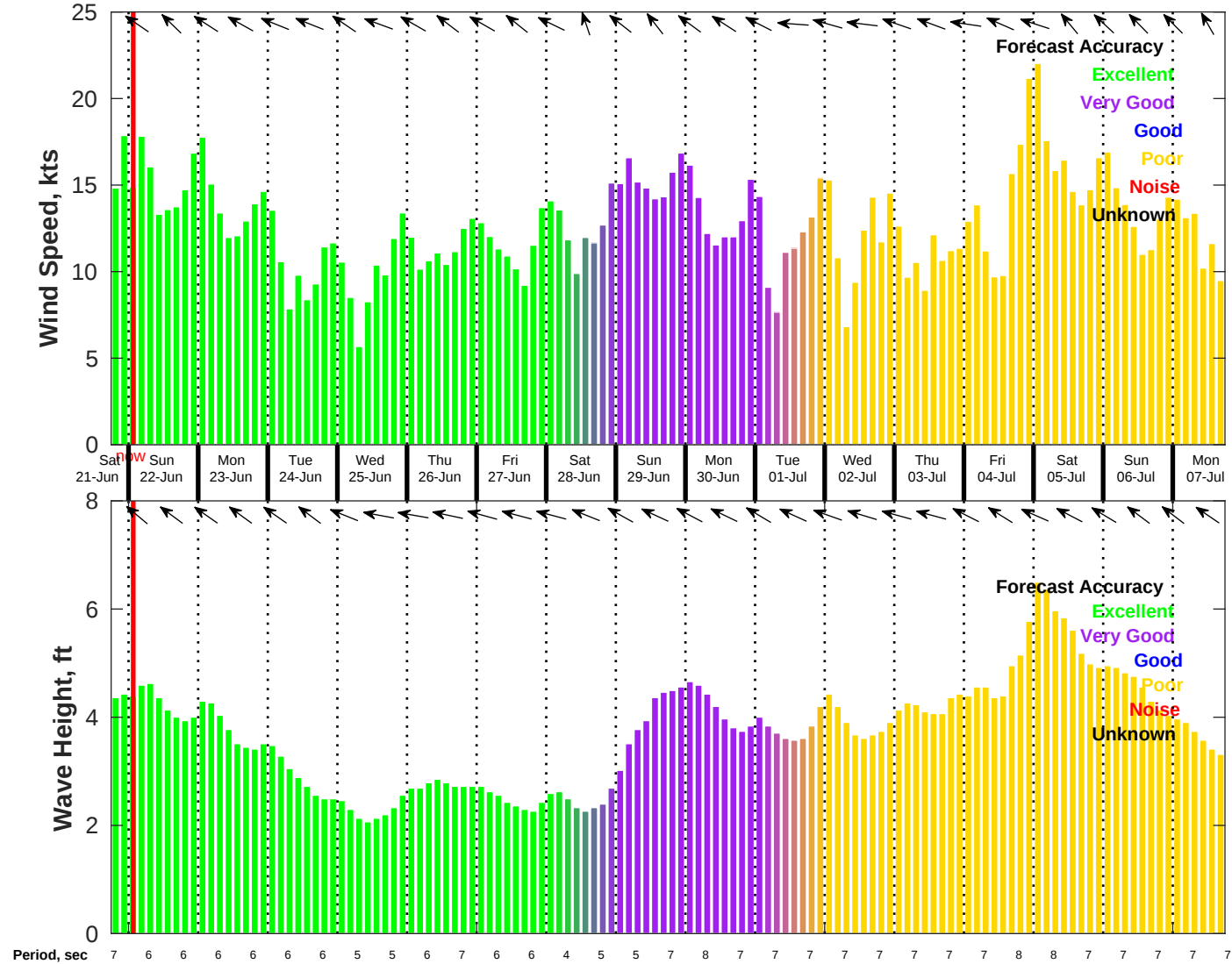
Wind & Wave Forecast for NDBC 42020 from 21-Jun-2025 18:00:00 to 07-Jul-2025 18:00:00
