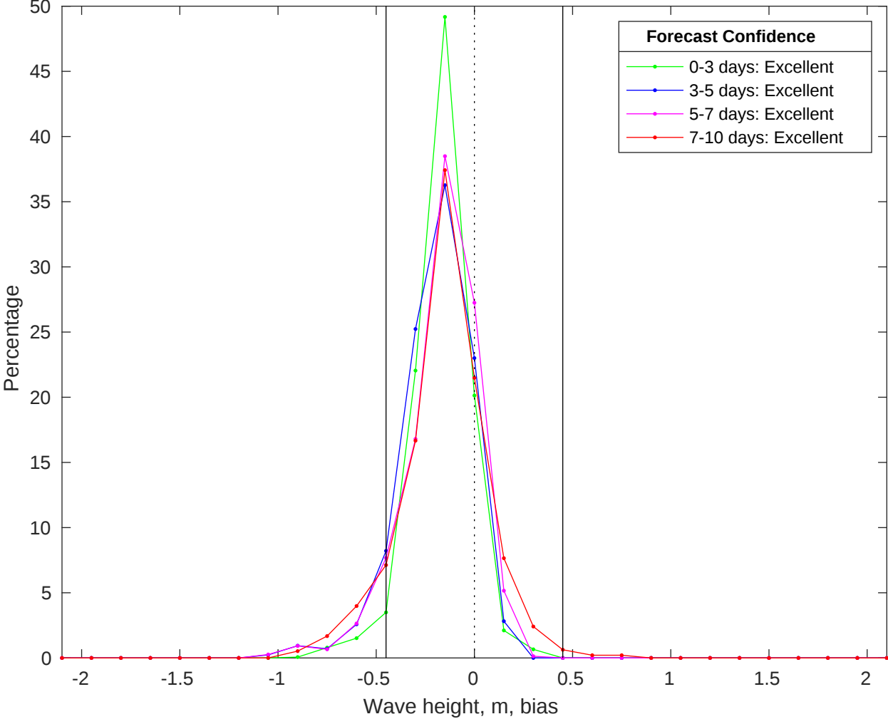
NDBC 42035 vs CMEMS Waves Bias Histogram: 22-Jun-2025
