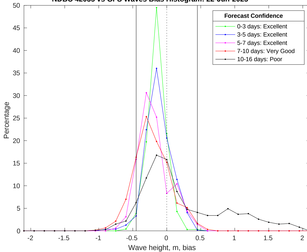
NDBC 42035 vs GFS Waves Bias Histogram: 22-Jun-2025
