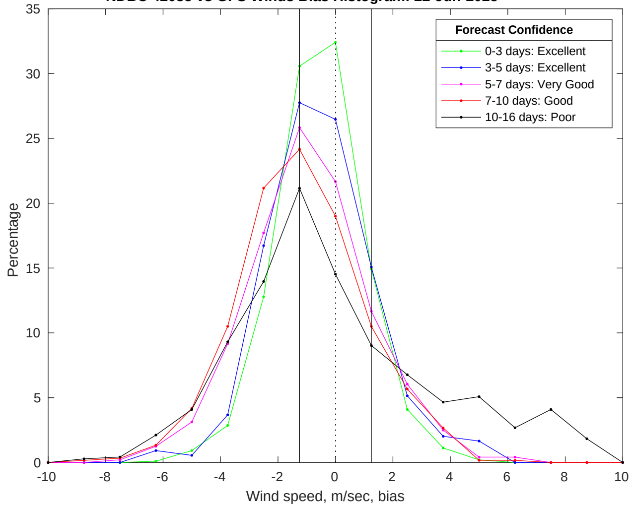
NDBC 42035 vs GFS Winds Bias Histogram: 22-Jun-2025
