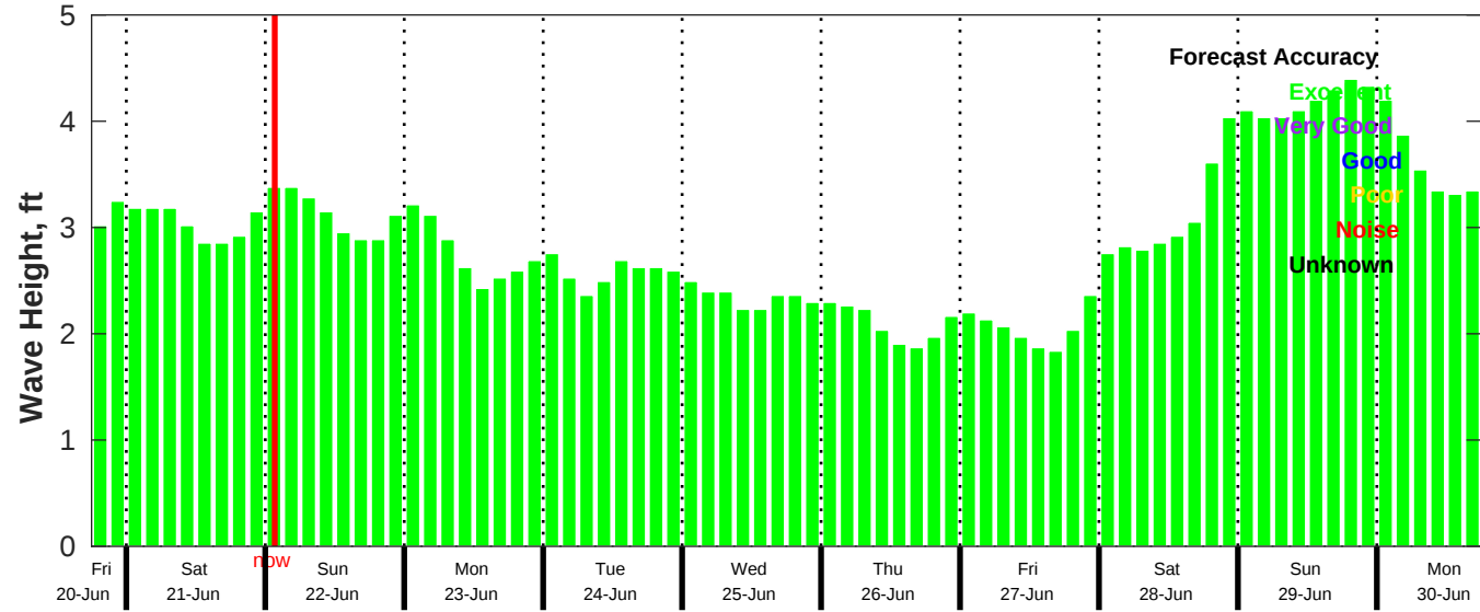
CMEMS Wave Forecast for NDBC 42035 from 20-Jun-2025 18:00:00 to 30-Jun-2025 18:00:00
