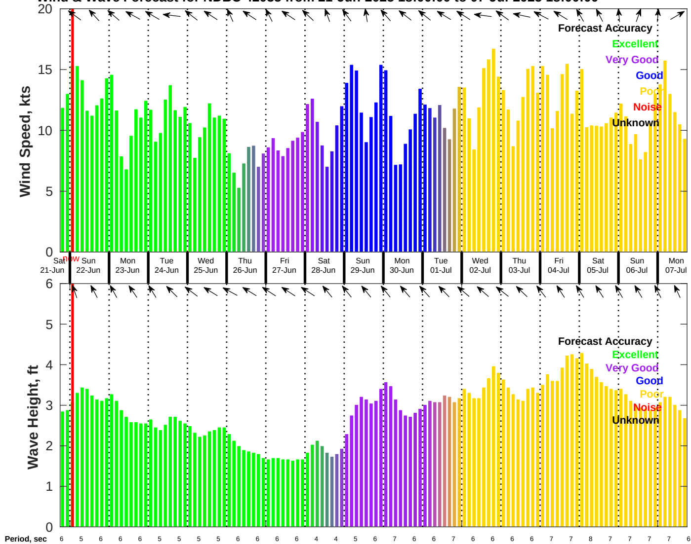
Wind & Wave Forecast for NDBC 42035 from 21-Jun-2025 18:00:00 to 07-Jul-2025 18:00:00
