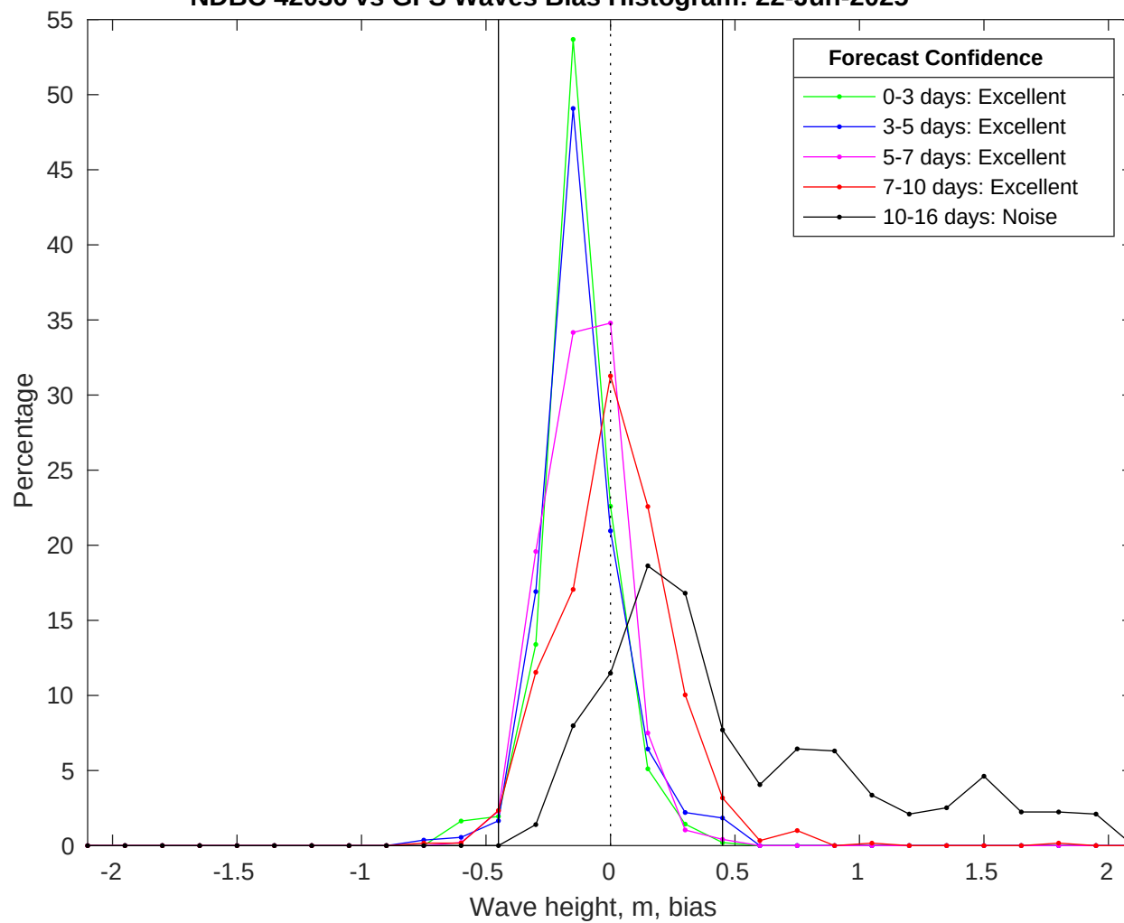
NDBC 42036 vs GFS Waves Bias Histogram: 22-Jun-2025
