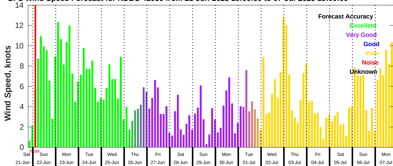
GFS Wind Speed Forecast for NDBC 42036 from 21-Jun-2025 19:00:00 to 07-Jul-2025 19:00:00
