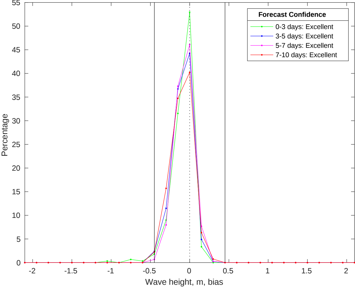
NDBC 42040 vs CMEMS Waves Bias Histogram: 22-Jun-2025
