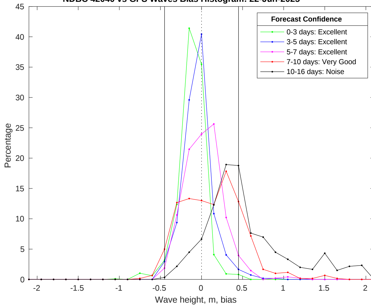
NDBC 42040 vs GFS Waves Bias Histogram: 22-Jun-2025
