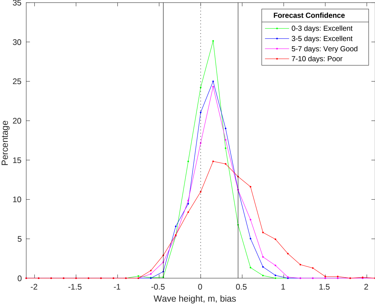
NDBC 46011 vs CMEMS Waves Bias Histogram: 22-Jun-2025
