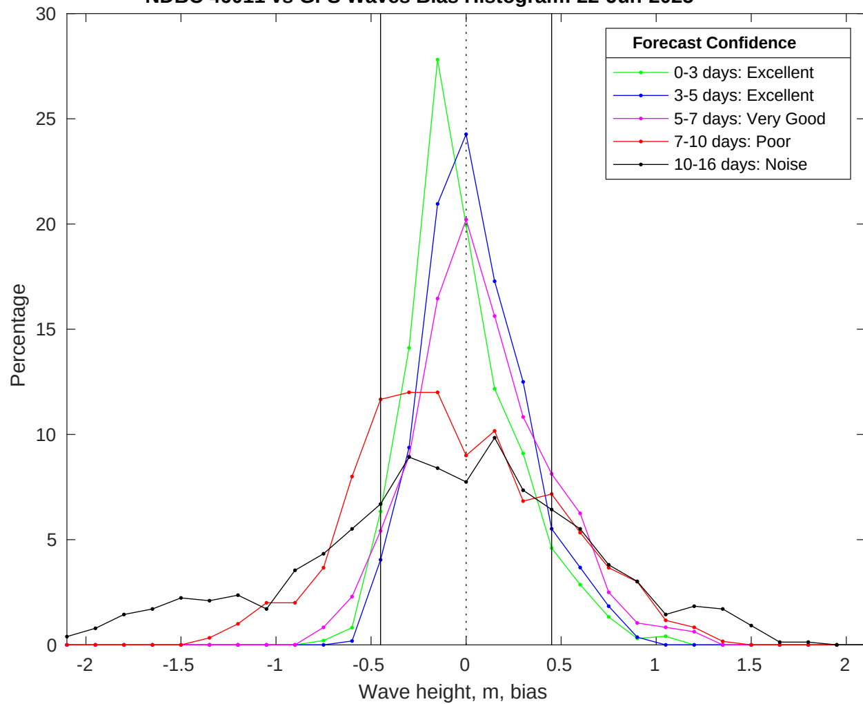
NDBC 46011 vs GFS Waves Bias Histogram: 22-Jun-2025
