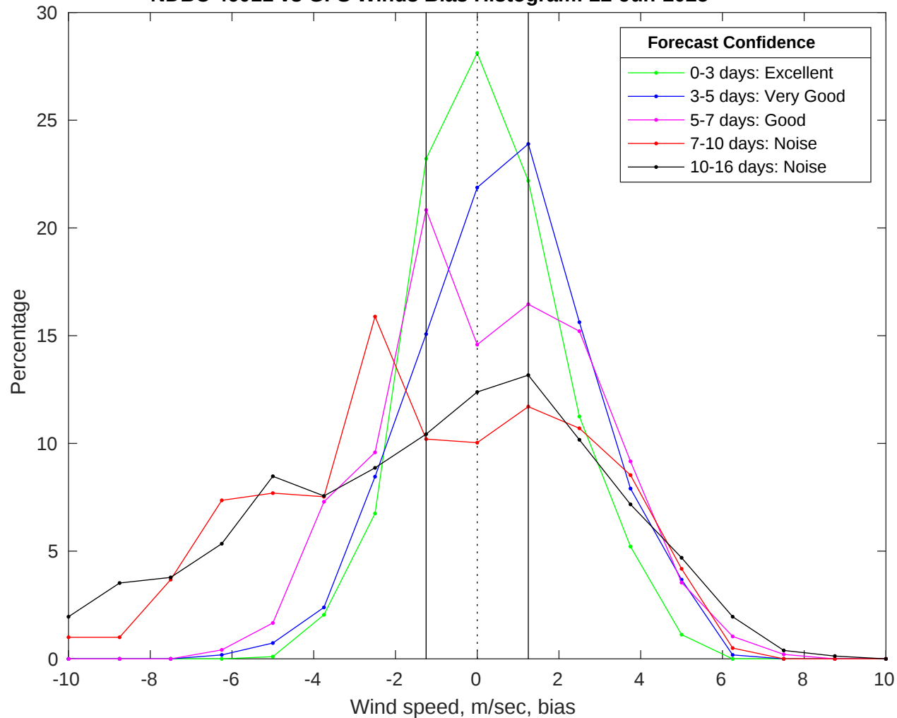
NDBC 46011 vs GFS Winds Bias Histogram: 22-Jun-2025
