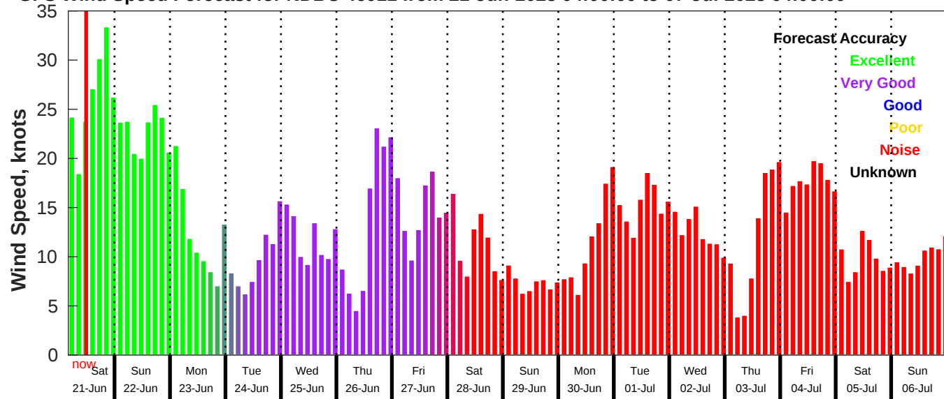
GFS Wind Speed Forecast for NDBC 46011 from 21-Jun-2025 04:00:00 to 07-Jul-2025 04:00:00
