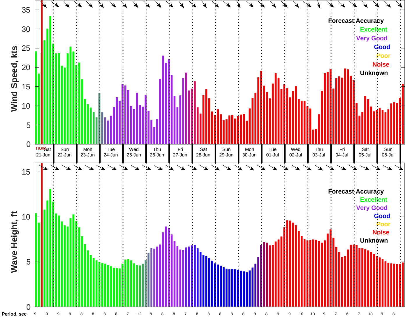
Wind & Wave Forecast for NDBC 46011 from 21-Jun-2025 04:00:00 to 07-Jul-2025 04:00:00
