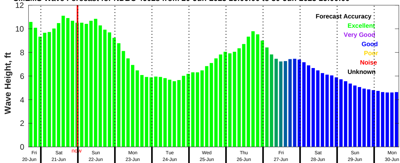
CMEMS Wave Forecast for NDBC 46028 from 20-Jun-2025 16:00:00 to 30-Jun-2025 16:00:00
