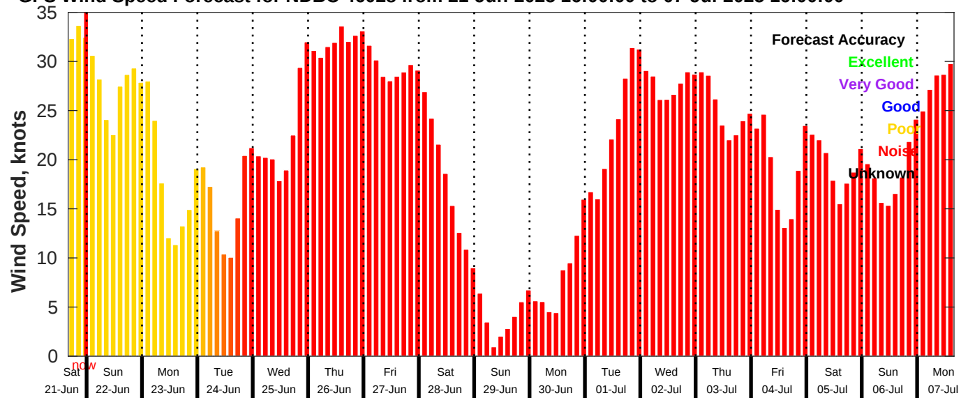
GFS Wind Speed Forecast for NDBC 46028 from 21-Jun-2025 16:00:00 to 07-Jul-2025 16:00:00
