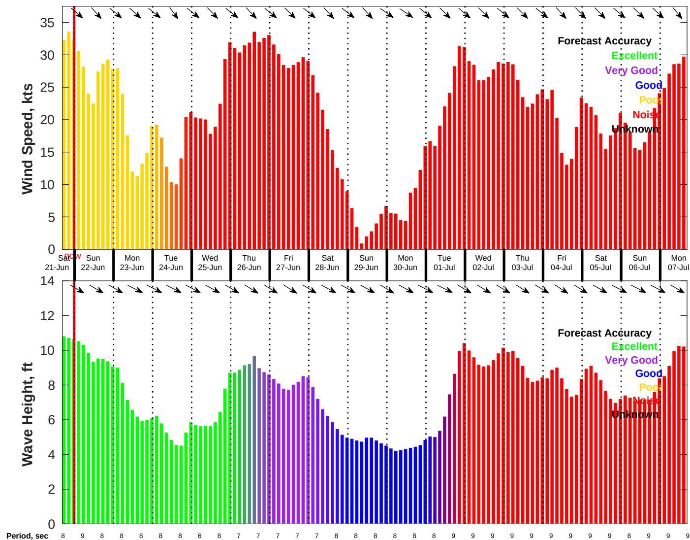
Wind & Wave Forecast for NDBC 46028 from 21-Jun-2025 16:00:00 to 07-Jul-2025 16:00:00
