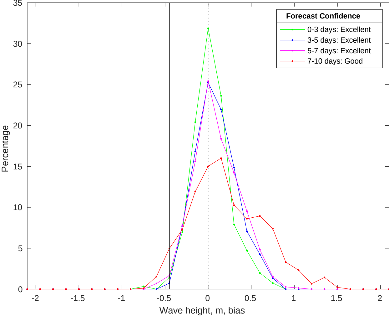
NDBC 46054 vs CMEMS Waves Bias Histogram: 22-Jun-2025
